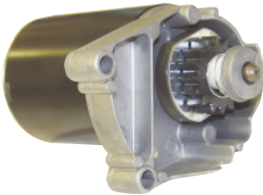
01-5528 12 V - 16h = 393017, 394674, 394808, 110635, - Briggs & Stratton, John Deere...
