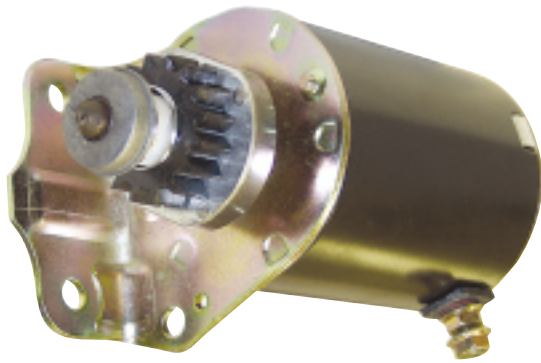
01-5527 12 V - 16h = 392749/R, 390838, 391423, US851... - Briggs & Stratton, Cub Cadet, Toro
